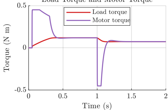
Load Torque and Motor Torque
